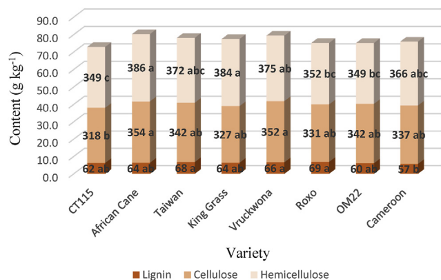
Fig. 3. Lignin (ADL), cellulose (ADF-ADL) and hemicellulose content (NDF-ADF) in the whole plant for eight varieties of Cenchrus purpureus at day 185 after planting. Means with different letter within the same fraction show statistical difference (Tukey test, P < 0.05 ).
